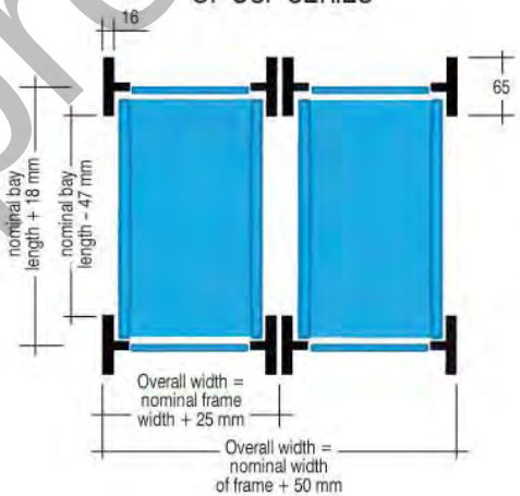
DIMENSIONS FOR THE DESIGN OF USP SERIES
